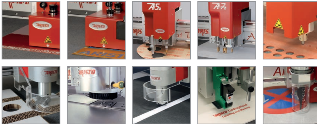
Oscillating cutting, creasing, V-cutting, routing, wheel cutting, labelling, marking, punching ...
